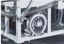
配备大功率高压旋涡风机，吸风效果强，噪音低 配备低隔断式吸风装置箱，灵活切换进行吸附面料的工作 Equipped with High Power and Pressure Swirl Air Blower, Strong Sucking Effect, Low Noise, Partitioned Sucking Device Box, Flexible Switching for Suction of Fabrics.
