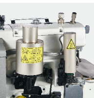
电磁铁剪线抬压脚 Electromagnet thread cutting and presser foot lifting
