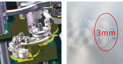
超短线头3mm Ultra Short Thread Remaining Length of 3mm
