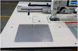
超密封窝吸风板，吸风渗透性更强。 Ultra-dense honeycomb air suction plate, stronger air permeability.
